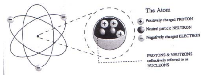
Structural motion of an atom
