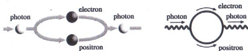
The creation of virtual photon at low energy (Qi) level
