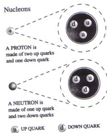
Quark composition of a Proton and a Neutron
